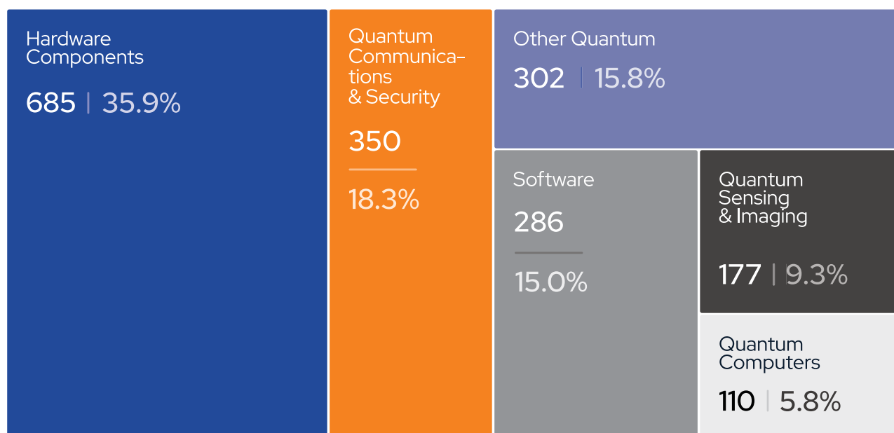
Figure 6: Distribution of 1,910 quantum companies by segment through Q1 2026.
